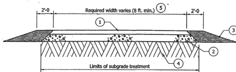
HMA TYPICAL SECTION
