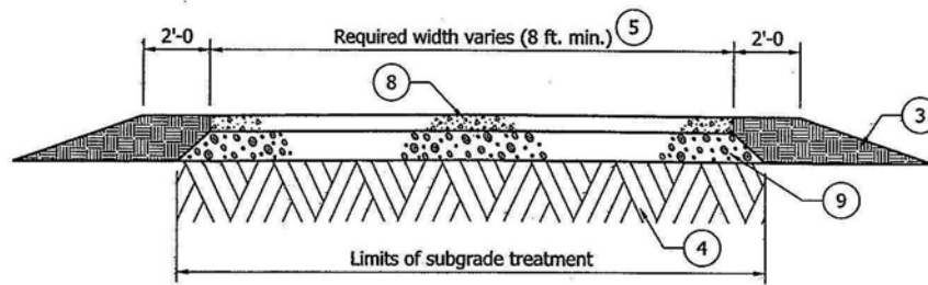
PCCP TYPICAL SECTION
